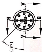
BACK VIEW
